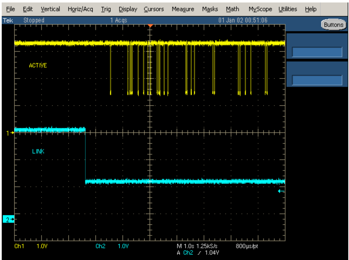
Figure 1.4-3 100M cable plugged-in of LINK/ACTIVE LEDs
