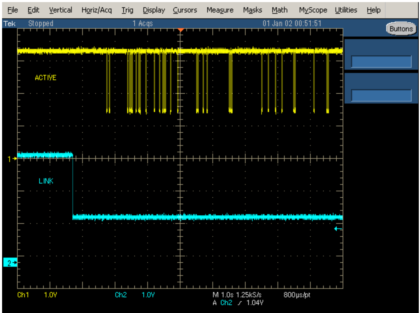
Figure 1.4-4 1000M cable plugged-in of LINK/ACTIVE LEDs
